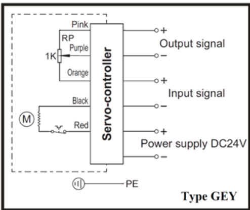
DC Voltage Wiring Diagram
