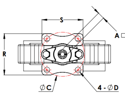
3" ISO 5211 mounting
